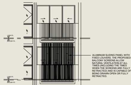
TYPICAL RETRACTABLE BALCONY SCREEN (CLOSED) - ELEVATION 1
