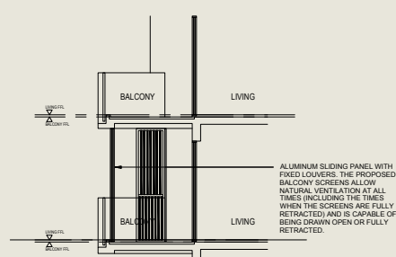
TYPICAL RETRACTABLE BALCONY SCREEN - SECTION A-A
