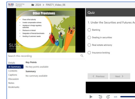
Interactive learning
