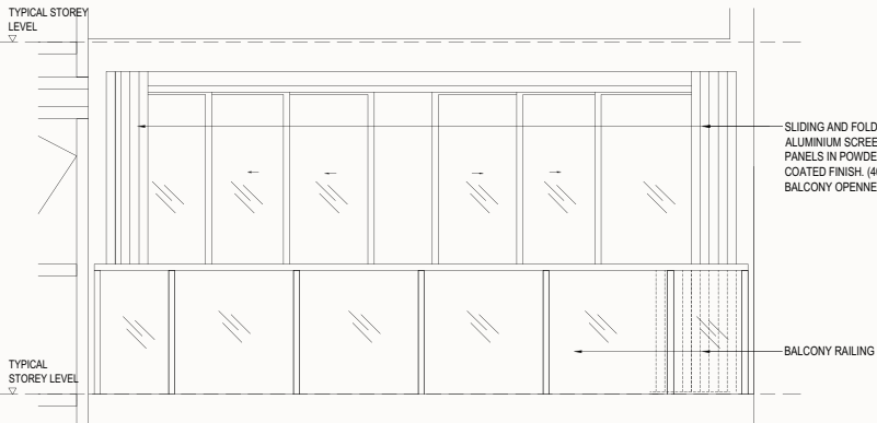
BALCONY/ PES SCREEN - FRONT ELEVATION (External View) When Screen is Opened
