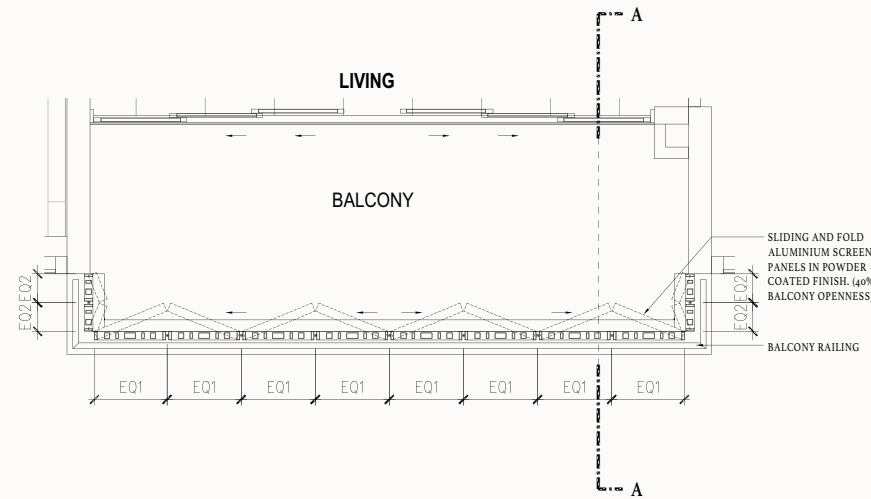
BALCONY/ PES SCREEN - PLAN
