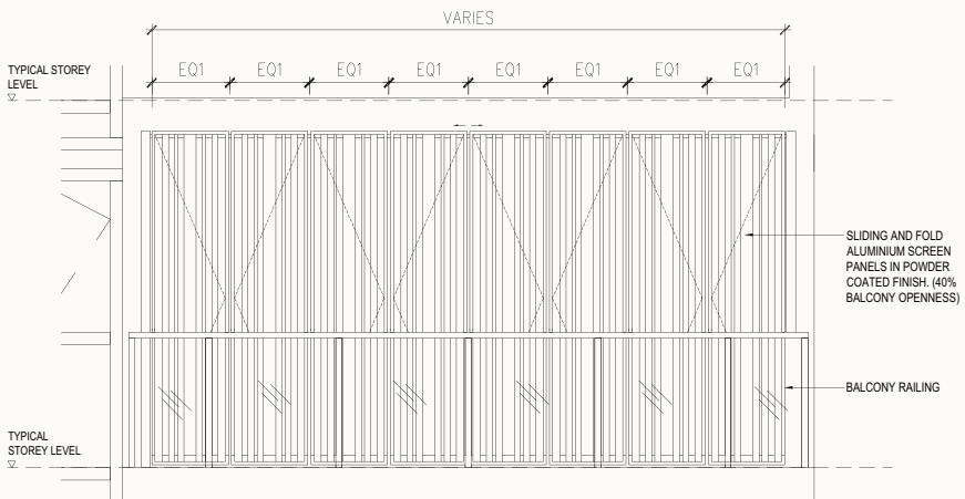
BALCONY/ PES SCREEN - FRONT ELEVATION (External View) When Screen is Closed
