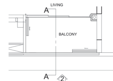
#44-01, #44-02, #44-04, #44-06, #44-08, #44-09, #44-10, #44-11, #44-12: TYPICAL RETRACTABLE BALCONY SCREEN (OPEN) - PLAN
