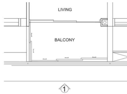
23RD TO 33RD STOREY (APPLICABLE TO ALL TYPES EXCEPT TYPE A1 AND A2) , 35TH TO 43RD STOREY (APPLICABLE TO ALL TYPES EXCEPT TYPE A1 AND A2) AND #44-03: TYPICAL RETRACTABLE BALCONY SCREEN (CLOSED) - PLAN
