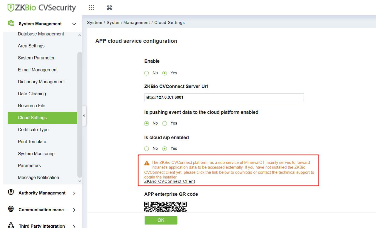
Figure 2 ZKBio CVSecurity System Management
