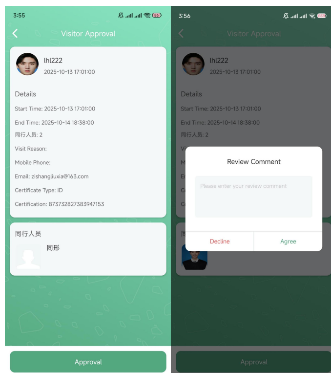
Figure 64 Agree or Decline
